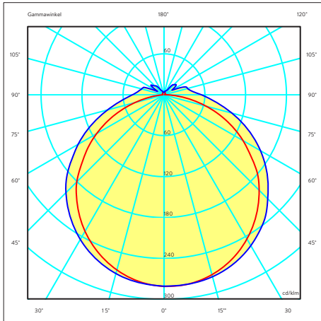
Lichtverteilungskurve DIAMANT FIT5 E-Line 30-72 W, 140° light emitting diag. DIAMANT FIT5 E-Line 72 W, 140°
