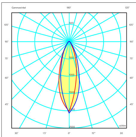
Lichtverteilungskurve DIAMANT FIT5 E-Line 30-72 W, 30° light emitting diag. DIAMANT FIT5 E-Line 30-42W, 30°
