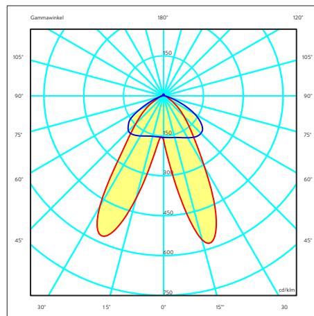
Lichtverteilungskurve DIAMANT FIT5 E-Line 30-72 W, 25° doppelt asymmetrisch light emitting diag. DIAMANT FIT5 E-Line 30-72W, 25° double asymmetrical
