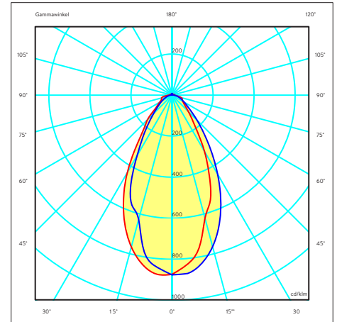
Lichtverteilungskurve DIAMANT FIT5 E-Line 30-72 W, 60° light emitting diag. DIAMANT FIT5 E-Line 30-42W, 30°
