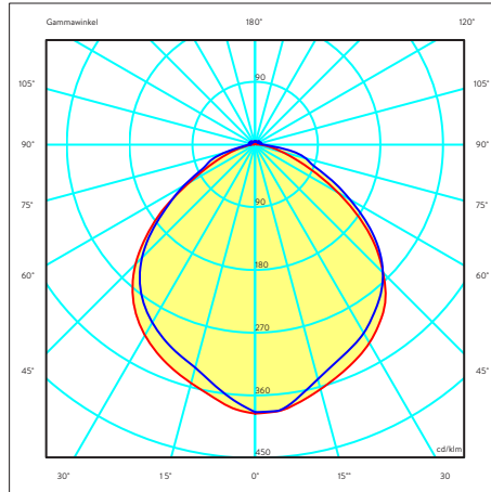
Lichtverteilungskurve DIAMANT FIT5 E-Line 30-72 W, 90° light emitting diag. DIAMANT FIT5 E-Line 72 W, 90°
